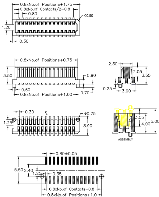
Recommended P.C.B Layout(Top Side)
