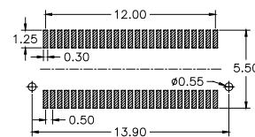
Recommended P.C.B Layout(Top Side)
