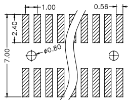
Recommended P.C.B Layout(Top Side)
