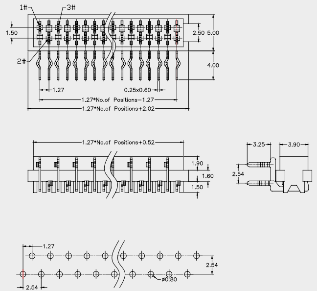
Recommended P.C.B Layout(Top Side)
