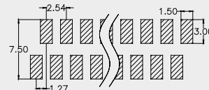
Recommended P.C.B Layout (Top Side)
